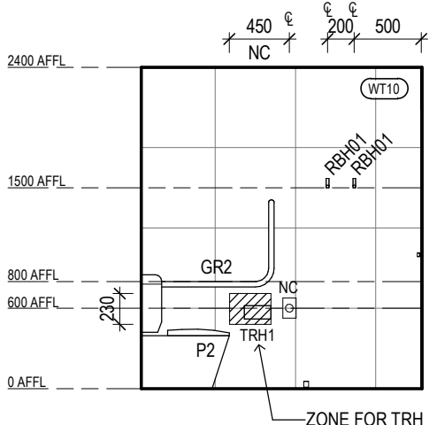
RACF STANDARD ROOM ENSUITE ELEVATION 2 Scale 1 : 50
